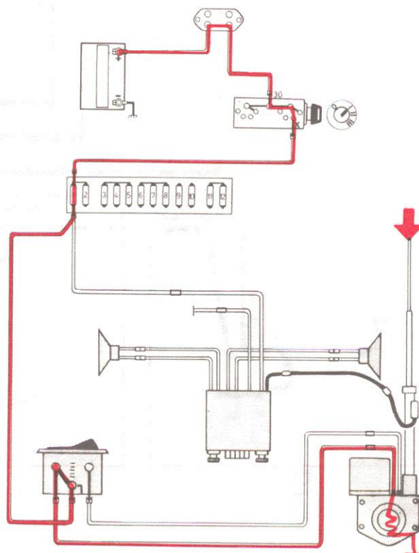
Power antenna being lowered
