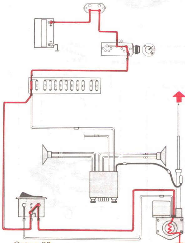
Power antenna being raised
