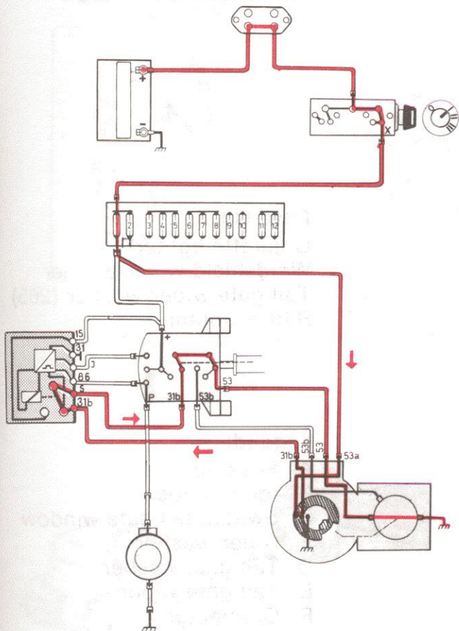
Washer operation (with wiper operating)
