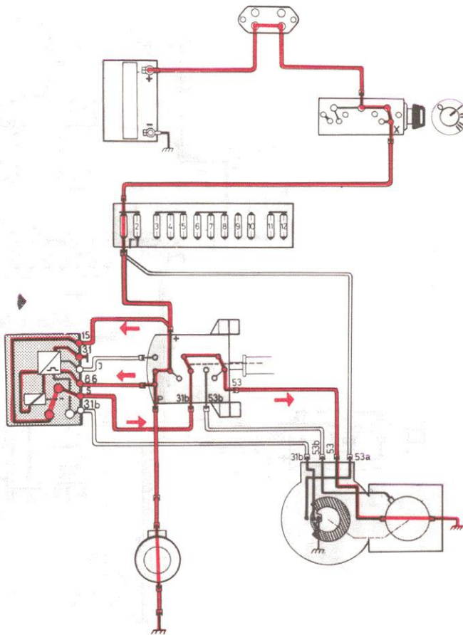
Parking (circuit during the last stroke)
