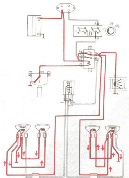
Headlight flasher
