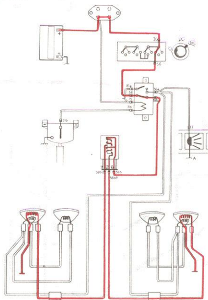
Lower beam
