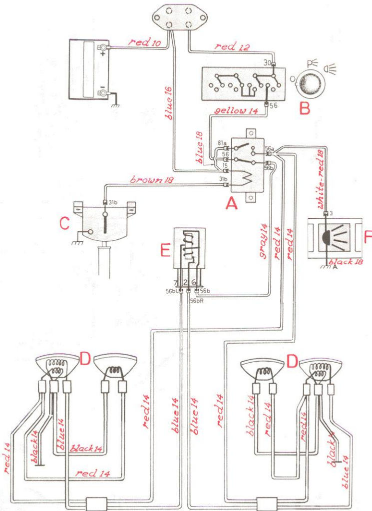
Upper beam
