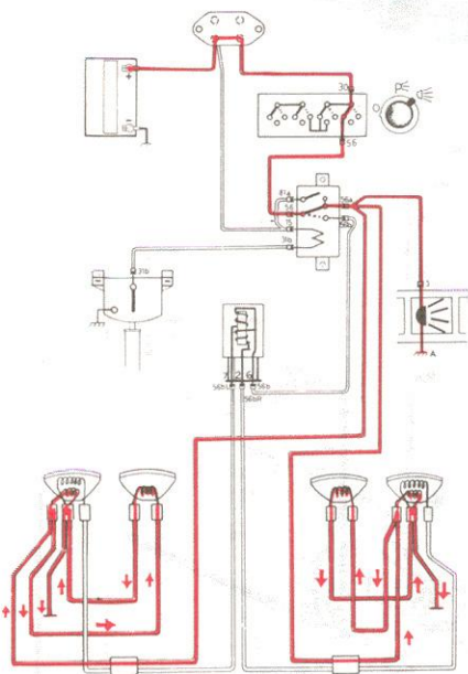
Upper beam
